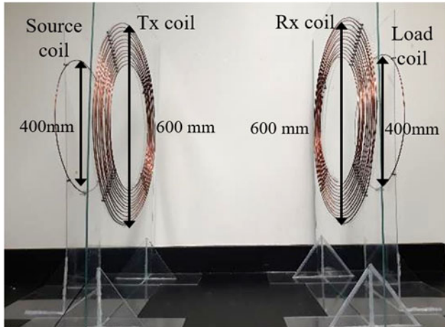
Fig. 5. Fabricated four-coil WPT system.
