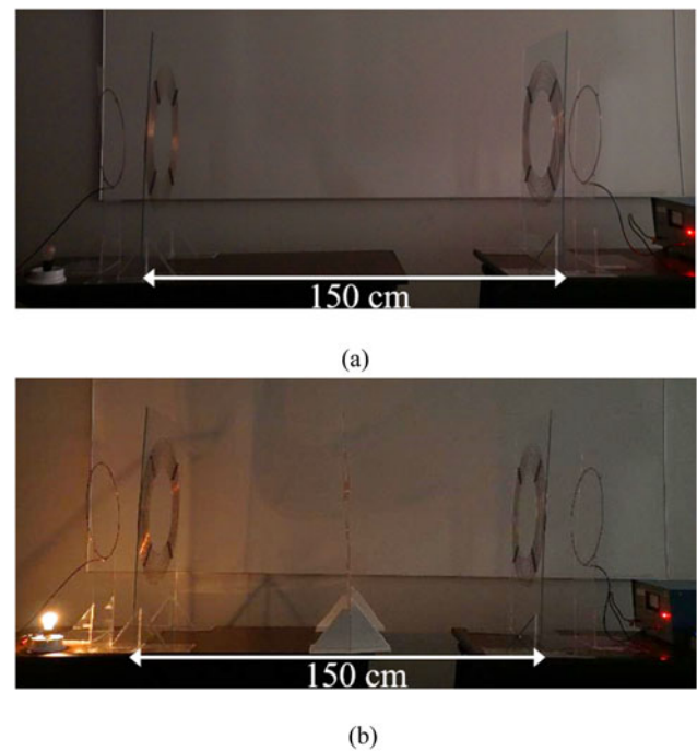
Fig. 11. The intensity of the light bulb connected to the WPT system at a distance 150 cm: (a) without metamaterial, and (b) with metamaterial.
